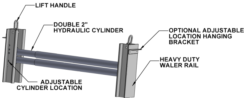
HYDRAULIC STRUT PSH-HS2
