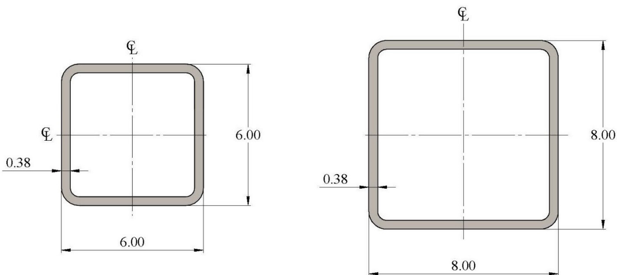
Figure 3. Square Tubing Specifications
