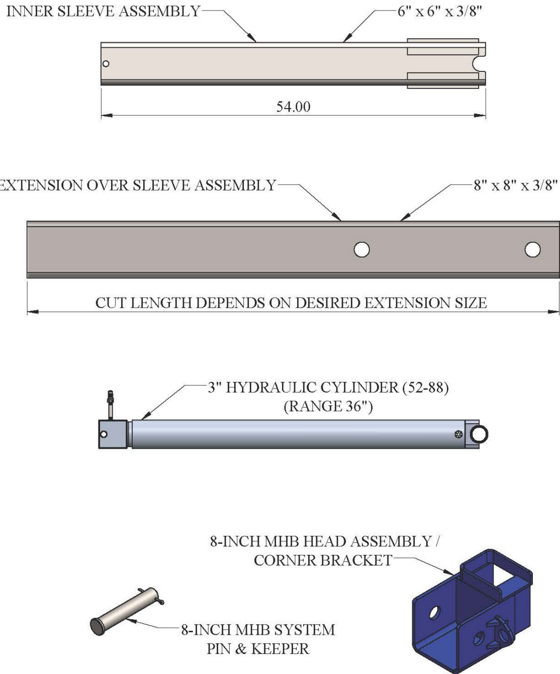
Figure 1. Components
