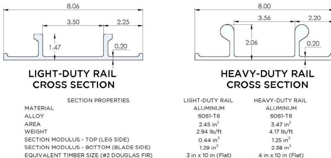
Figure 7: Vertical Rail Specifications
