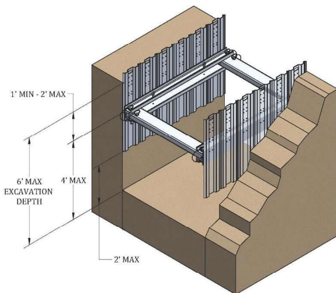
Figure 3. Single Waler Use
