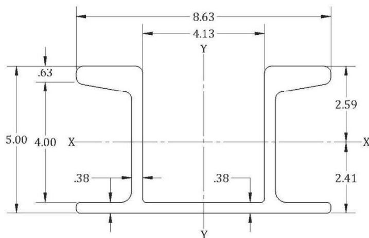
Figure 6. Heavy-Duty Waler Rail
