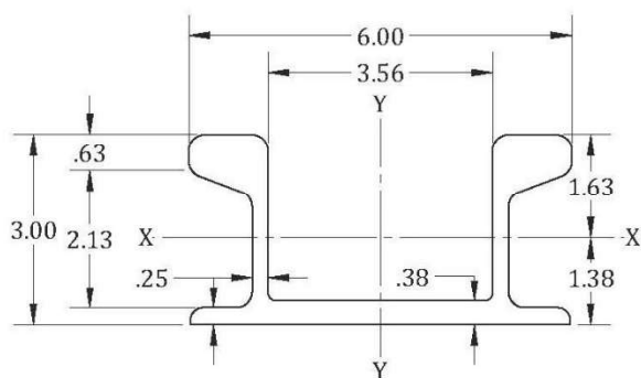
Figure 5. Light-Duty Waler Rail
