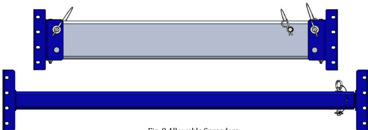
Fig. 8 Allowable Spreaders
