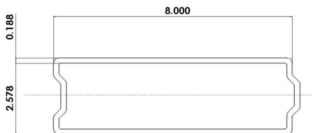
Fig. 4 Section Properties
