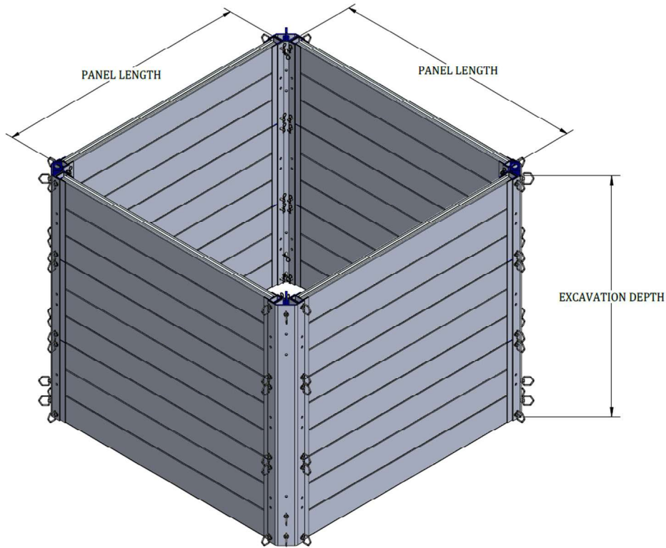
Fig. 5 Four-Sided Application
