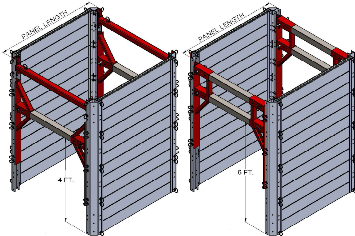
Fig. 9 High Clearance Arches
