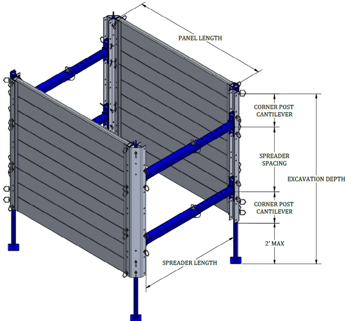
Fig. 7 Two-Sided Application
