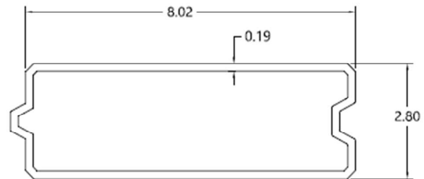
BUILDABLE BOX PANEL
